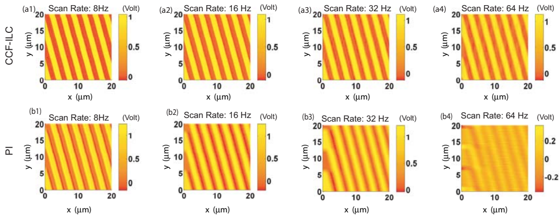
Figure 5.4 Comparison of the sample estimation results by using by using (the upper row) the proposed CCF-ILC approach with that by using (the bottom row) the PI control for four different equivalent scan rates of (a1, b1) 8Hz, (a2, b2) 16Hz, (a3, b3) 32Hz, and (a4, b4) 64Hz. The effective lateral scan range was assumed as 20 \mu\text{m} .
