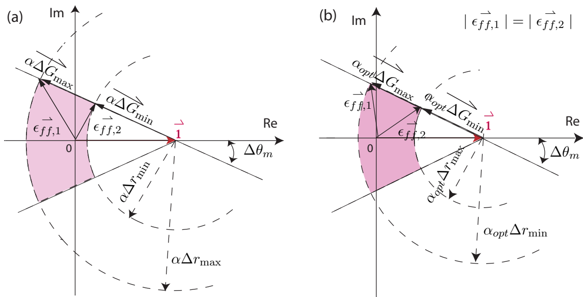
Figure 3.2 The geometric interpretation of the robust-system-inversion method: (a) the feedforward gain-error (shaded area) for the dynamics uncertainties bounded by \Delta r_{\min} , \Delta r_{\max} , and \Delta\theta_m , with an arbitrarily chosen gain coefficient \alpha , and (b) the minimized gain-error for the optimal gain coefficient \alpha_{opt} .
